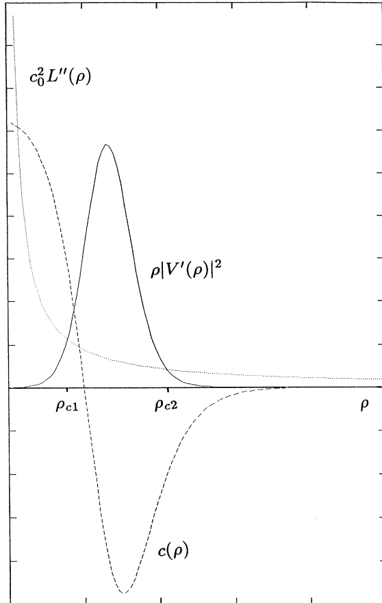
FIG. 1. The two terms \rho |V'(\rho)|^2 (solid curve) and c_0^2 L''(\rho) (dotted curve) in the stability criterion (7). The intersections of these two curves locate the critical densities \rho_{c1} and \rho_{c2} . The dashed curve is the velocity c(\rho) from Eq. (9). Note that c' is negative at \rho_{c1} and positive at \rho_{c2} . All curves are calculated for the functions V'(\rho) = -21.025 \text{sech}^2[(\rho - 0.25)/0.12] and L(\rho) = \ln \rho and the value c_0 = 2.48445 used in Ref. [3].
